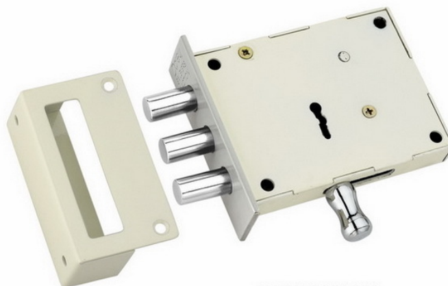
SLEEK DOOR LOCK 2 IN 1 BULLET PC/CP 75 x 100 x 17.5mm KY
